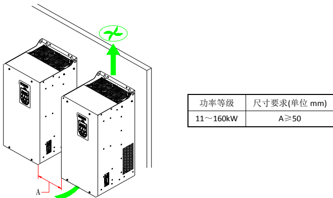
图3-3 Hope130G11T4~Hope130G160T4多台机器并排安装
